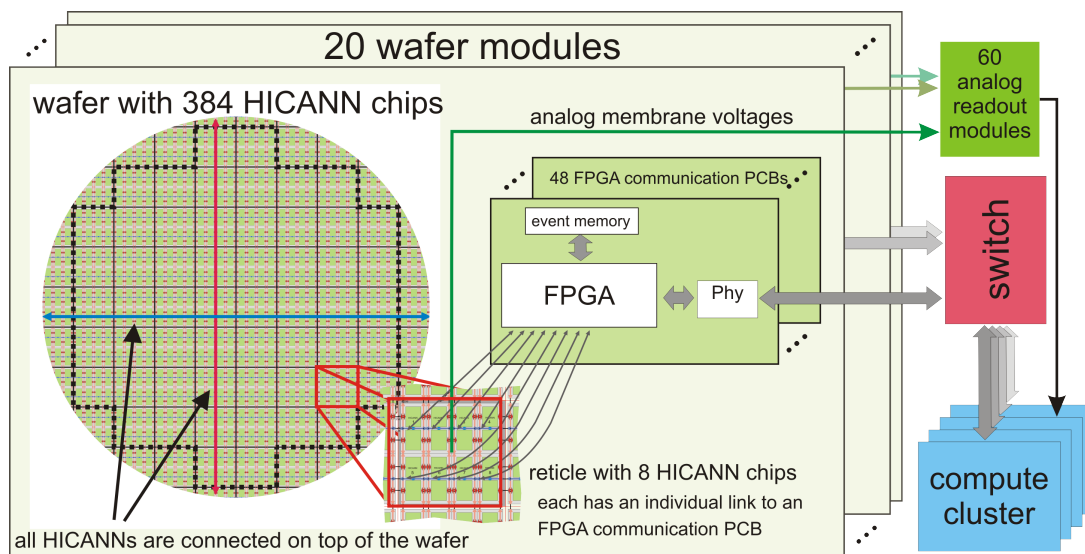
Figure 2.1.1: Simplified overview of the Neuromorphic Physical Model version 1 (NM-PM1) system.
